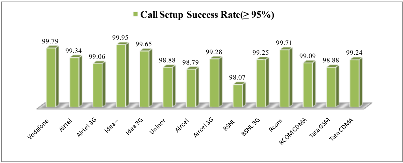
Fig. 3 According to the above graph and data on the table, it is found that all the operators are meeting the Network Parameters.
