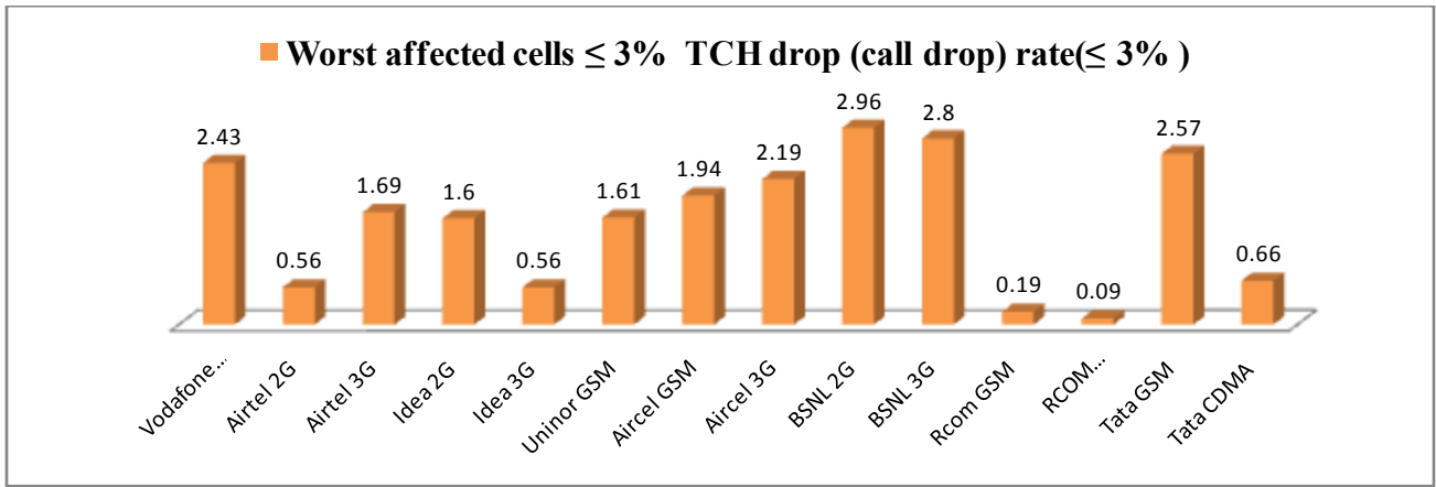
Fig.7 According to the above graph and data on the table, it is found that all the operators are meeting the Network Parameters.
